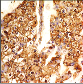
Fig-1: Immunohistochemical analysis of B7-H4 antibody in Renal cell carcinoma using anti-B7-H4 antibody (Clone: ABM53A6) at 5 \mu g/ml
