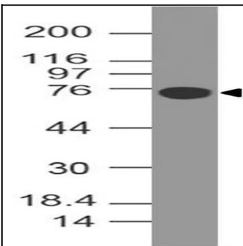
Fig-3: Western blot analysis of B7H4. Anti-B7H4 antibody (Clone: ABM53A6) was used at 4 \mu g/ml on human B7H4-FC fusion protein Lysate.
