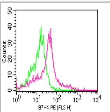
Fig-2: Cell surface Flow analysis of B7-H4 antibody in human PBMC (Monocytes) cells using 0.5 \mu g/ 10 6 cells of anti-B7-H4 antibody (ABM53A6). Green represents isotype control; red represents anti-B7H4 antibody. Goat anti-mouse PE conjugate was used as secondary antibody.
