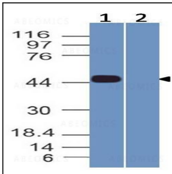
Figure-5: Western Blot analysis of SARS-CoV-2 Nucleocapsid Antibody: Anti- SARS-CoV-2 Nucleocapsid Antibody (Clone: ABM4H11.1C12) was used at 4 µg/ml on (1) SARS-CoV-2 virus infected Vero Cell lysates and (2) Mock infected lysates.
