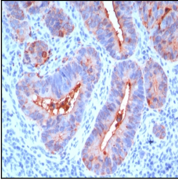
Formalin-fixed, paraffin-embedded human Colon Carcinoma stained with CEA Monoclonal Antibody (C66/195).
